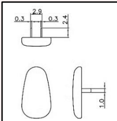
TPA-01T Material: Titanium
