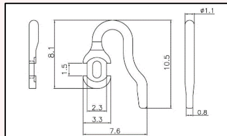
TPA-05HUG Material: Titanium
