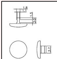
TPA-01NS Material: Nickel silver
