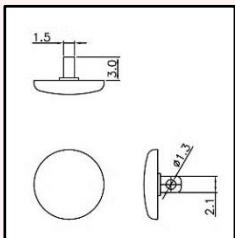
TPA-01NS Material: Nickel silver
