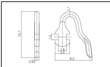
TPA-01T Material: Titanium
