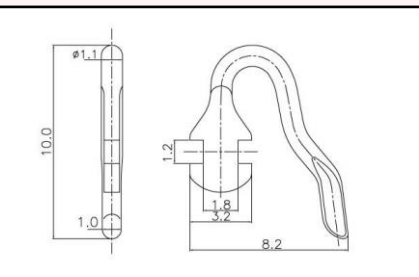
TPA-01NS Material: Nickel silver
